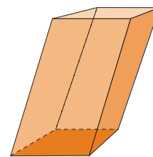
Prisma oblic
